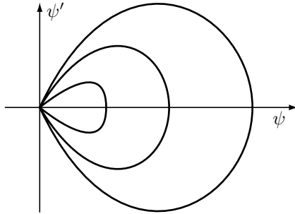
Figure 1.1. Phase plane portrait of \psi'' + \lambda \psi + |\psi|^{p-1}\psi = 0
