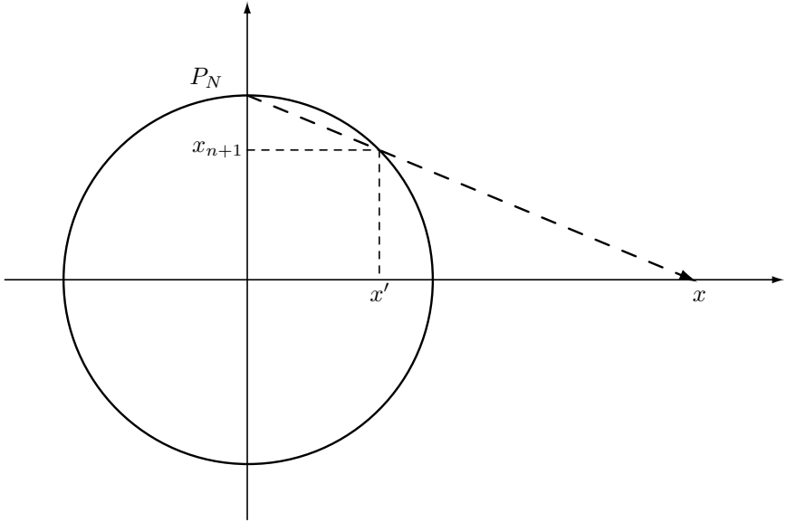
Figure 6.1. The stereographic projection ( x = \pi(x', x_{n+1}) )
